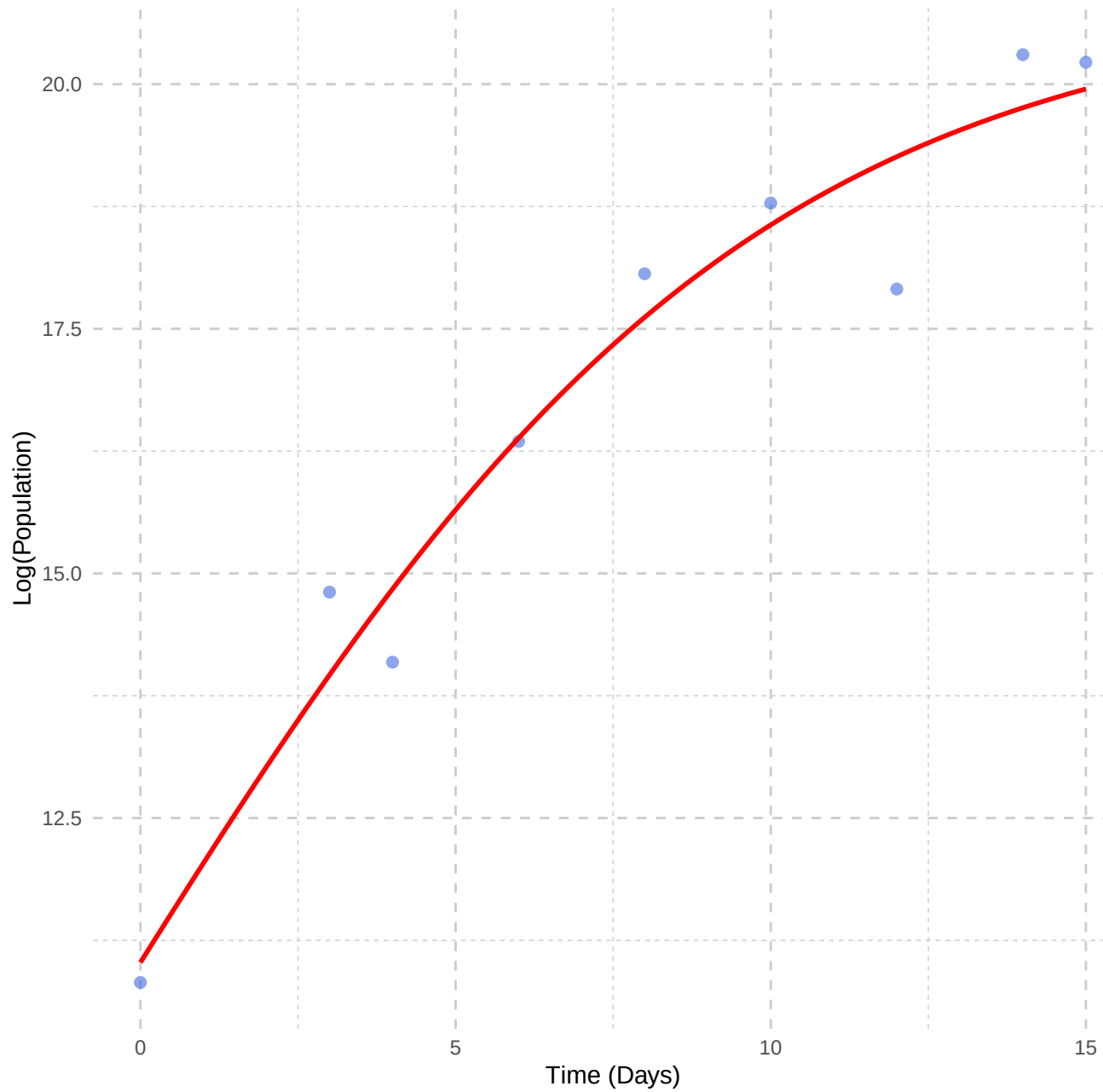
Bacterial Growth Curve Fit
